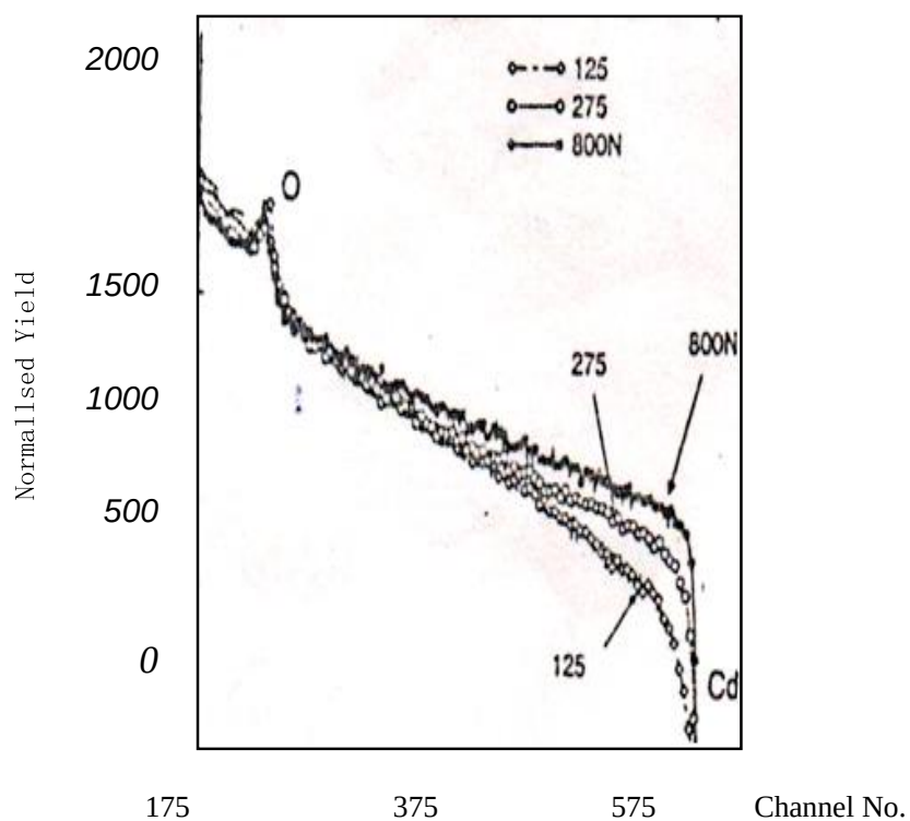
Fig.1 RBS spectrum for 3.05 MeV alphas on CdO
